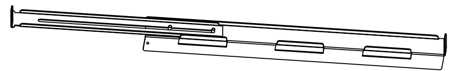
Maximum stroke 1090mm, right rail
